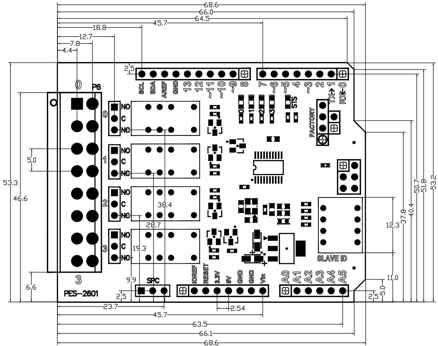
PES-2601 Dimension (mm)
